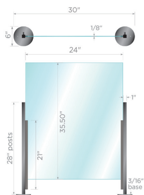
AC-SF-3624-SHIELD-BK 36"h x 24"w 6"w x 3/16"d base
