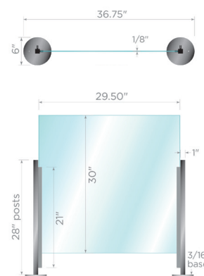
AC-SF-3030-SHIELD-BK 30"h x 30"w 6"w x 3/16"d base
