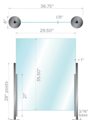
AC-SF-3630-SHIELD-BK 36"h x 30"w 6"w x 3/16"d base
